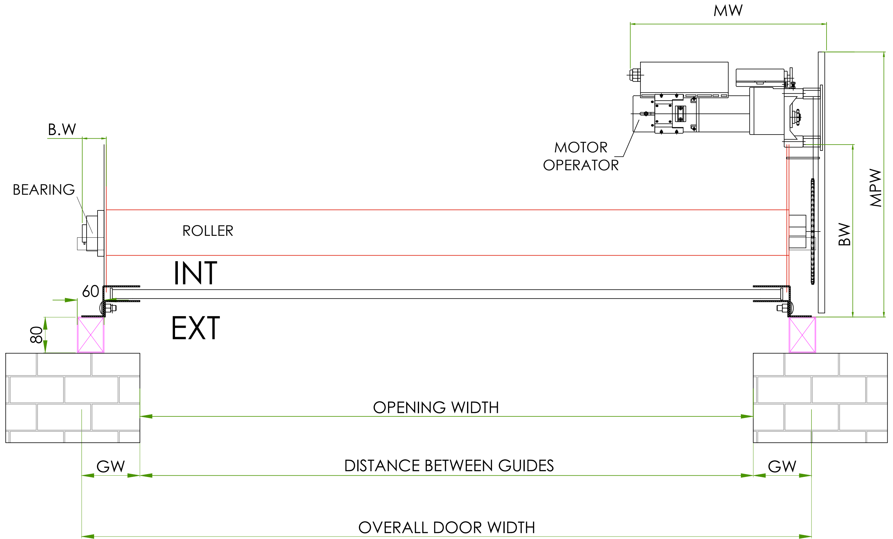
PLAN AT ROLLER LEVEL
